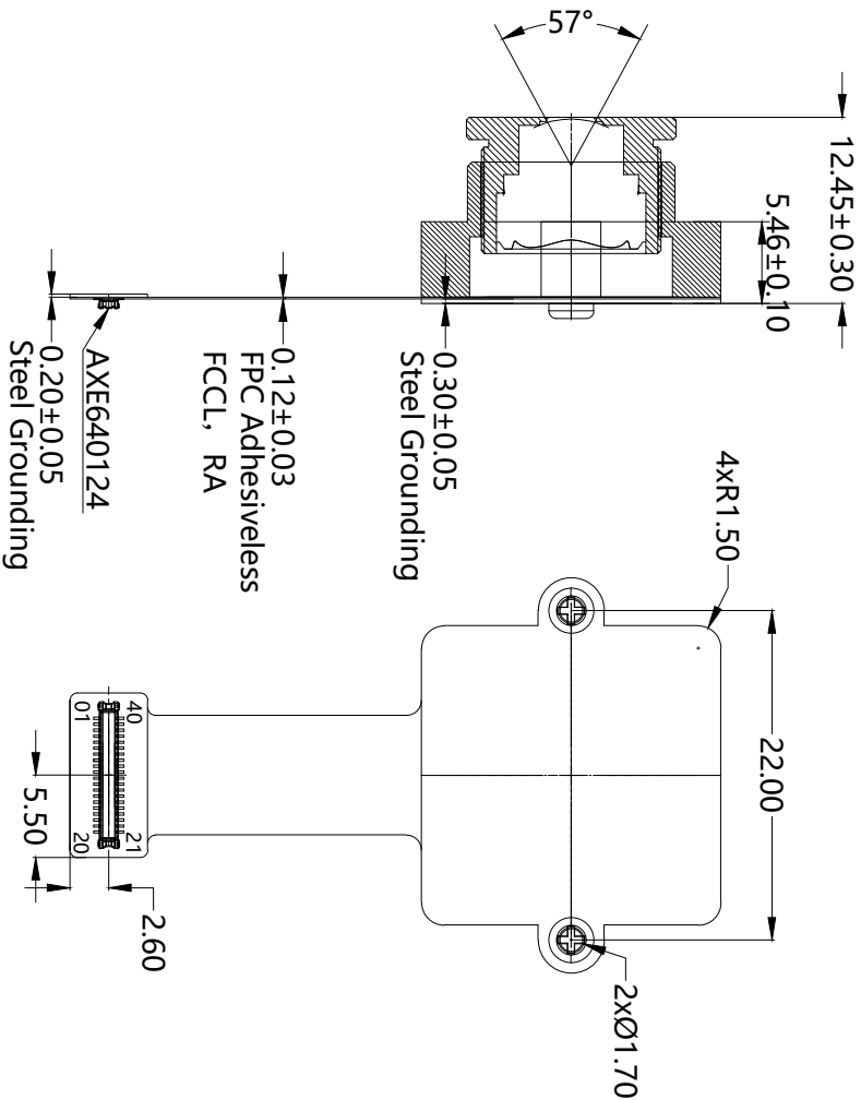
SIDE VIEW
